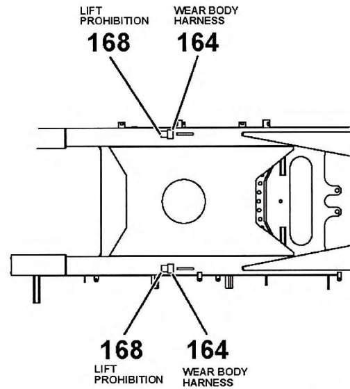
PARTIAL TOP VIEW OF S/S TURNTABLE
